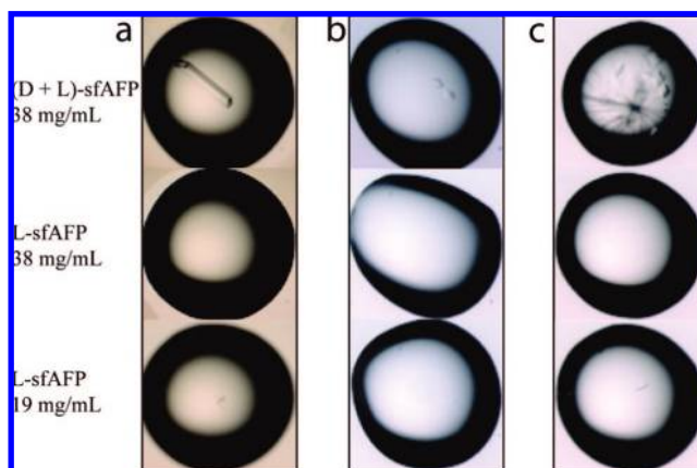
Figure 1. A direct comparison of the results for attempted crystallization of the racemic protein mixture [D-sfAFP + L-sfAFP] or the single enantiomer L-sfAFP under three sets of conditions. Protein crystals appeared rapidly from a solution containing a racemic mixture of D-sfAFP and L-sfAFP, but not for L-sfAFP alone, when screened under a standard set of crystallization conditions. Representative examples are shown in this Figure. X-ray diffraction was used to verify that the crystals were in fact protein. The crystallization conditions shown are a subset of the main findings reported here and are as follows: (a) 0.1 M bicine pH = 9.0, 2% v/v 1,4-dioxane, 10% w/v polyethylene glycol 20,000; (b) 0.1 M bis-Tris pH = 6.5, 1.15 M ammonium sulfate; (c) 0.1 M Tris pH = 8.5, 25% w/v polyethylene glycol 3350. All crystallization trials were carried out at room temperature (~23 °C).
