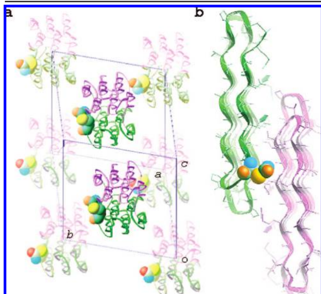
Figure 2. Quasi-racemate crystal packing in space group P1 , showing the D-sfAFP molecule (purple ribbon) and the L-sfAFP (green ribbon) with the “pseudo-Se-Gln” at position 11 shown as CPK solid spheres colored by atom type (C, green; O, red; N, cyan; Se, yellow). (a) Unit cell with two D-sfAFP/L-Se-sfAFP pairs located at positions 0 , 1/2b , 1/2c , and 0,0,0 , in the asymmetric unit. The D-sfAFP contains right-handed polyproline type II (PPII) helices; the L-sfAFP contains left-handed PPII helices. (b) View of one D-sfAFP/L-Se-sfAFP pair located at 0 , 1/2b , 1/2c . Side chains are included as stick representations.
