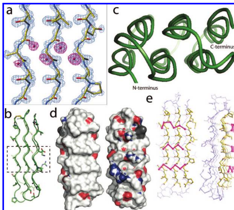
Figure 3. The X-ray structure of snow flea antifreeze protein (sfAFP). Atomic resolution ( 1.2 Å) X-ray structure of sfAFP, obtained from quasi-racemate crystals of D-sfAFP and L-Se-sfAFP in the P1 space group. (a) SigmaA-weighted 2F_o - F_c electron density map (blue, 1.5 sigma level) of the proposed ice-binding surface encompassing residues 17–21, 47–51, 74–78. Five ordered water molecules are shown (magenta spheres) with electron density shown at 1\sigma . (b) Cartoon of the backbone fold of sfAFP. Amino acid side chains are shown as sticks. The dashed box indicates the region shown in (a) above. (c) The main structural elements of sfAFP are six antiparallel polyproline type II (PPII) (left-handed) helices, stacked in two groups and joined by five reverse turns and interlocked by a complex hydrogen bond network. The N-terminal half of the protein contains two intramolecular disulfide bonds between residues Cys1–Cys28 and Cys13–Cys43. (d) Surface map highlighting sfAFP’s amphiphilic character. A 180^\circ rotation (along the long axis) shows the contrasting surfaces: hydrophobic/apolar (left); hydrophilic/polar (right). (e) Two views related by a 90^\circ rotation of highly ordered first shell water molecules (shown in magenta) interacting with the sfAFP hydrophobic face backbone (dashed magenta lines). Water molecules (magenta spheres) are within hydrogen-bonding distance ( 2.7 – 3.0 Å) of the sfAFP backbone amide carbonyls and nitrogens, and of one another (solid magenta lines). The spacing between water molecules is 4.5 Å and 9.2 Å along the short and long sfAFP axes, respectively. X-ray statistics are given in Table 1. Backbone rmsd deviations between molecules of L-sfAFP and D-sfAFP are given in Table 2.
