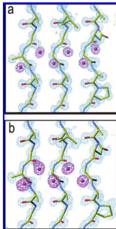
Figure 4. SigmaA-weighted 2F_o - F_c electron density map (blue, 1.5\sigma level) of the proposed ice-binding surface encompassing residues 17–21, 47–51, 74–78 for: (a) P2_1 L-sfAFP; (b) P\bar{1} {D-sfAFP + L-sfAFP}. Ordered water molecules with electron density at 1\sigma are shown (magenta spheres). Five ordered water molecules are conserved in all structures. An additional water molecule is observed in the P2_1 structure; this water is absent in the racemic crystals because of packing interactions.
