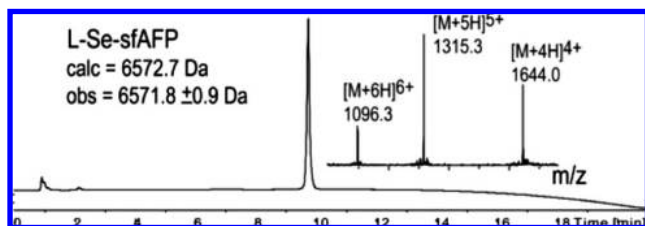
Figure 5. Analytical LC–MS data for synthetic folded L-Se-sfAFP. The chromatographic separations were carried out on a Vydac C4 2.1 mm × 150 mm column using a linear gradient of 1–61% buffer B over 15 min (buffer A = 0.1% TFA in H 2 O; buffer B = 0.08% TFA in acetonitrile). The inset is the ESMS summed over the entire LC peak. Calculated masses were based on average isotope composition.
